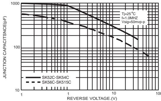
FIG.5-TYPICAL JUNCTION CAPACITANCE
