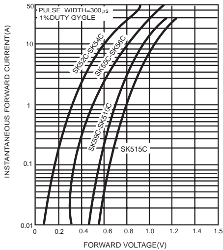
FIG.3-TYPICAL FORWARD CHARACTERISTICS
